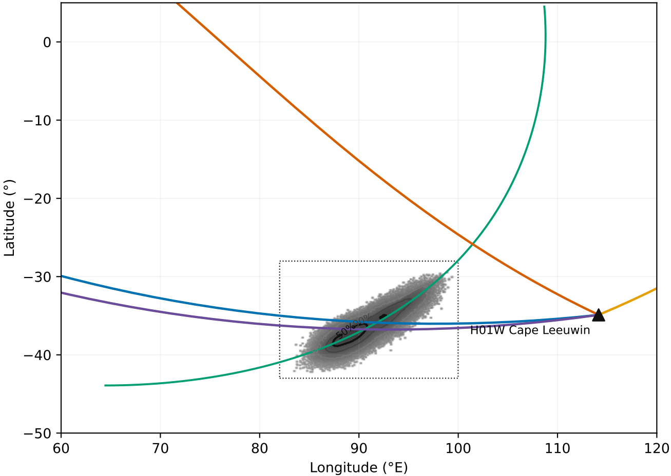
A. H01W source bearings against the seventh arc and integrated spatial PDF The preferred 306.18° line meets the arc well north of the integrated high-density area
