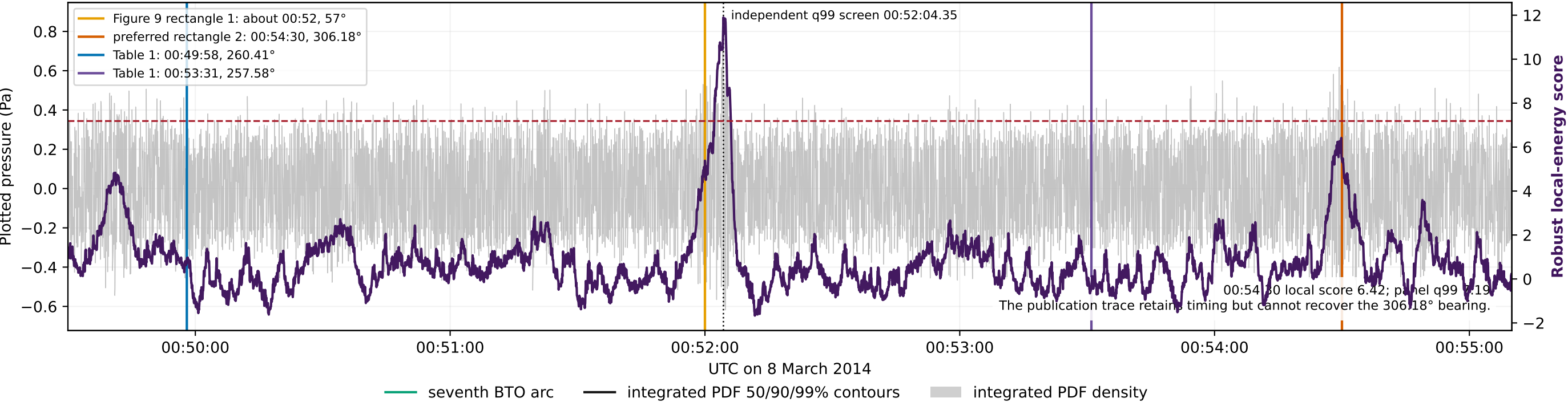
C. Figure 9c: light-grey pressure and high-contrast local-energy score at all noted source times
