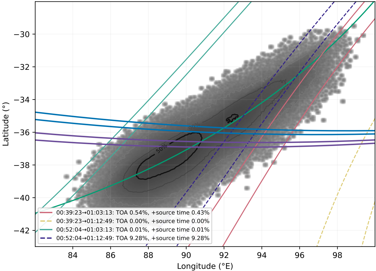
B. Independently screened H01W-H08S arrival-difference bands Percentages are integrated-PDF compatibility masses, not event probabilities
